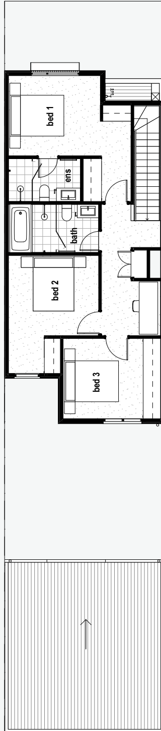
GROUND FLOOR
