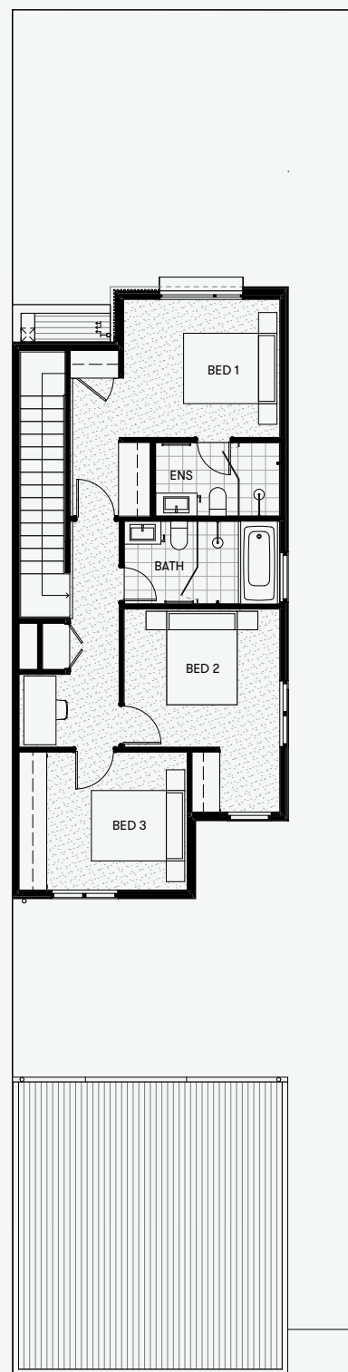
FIRST FLOOR
